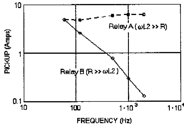
Figure 4: Pickup Current Versus Frequency
