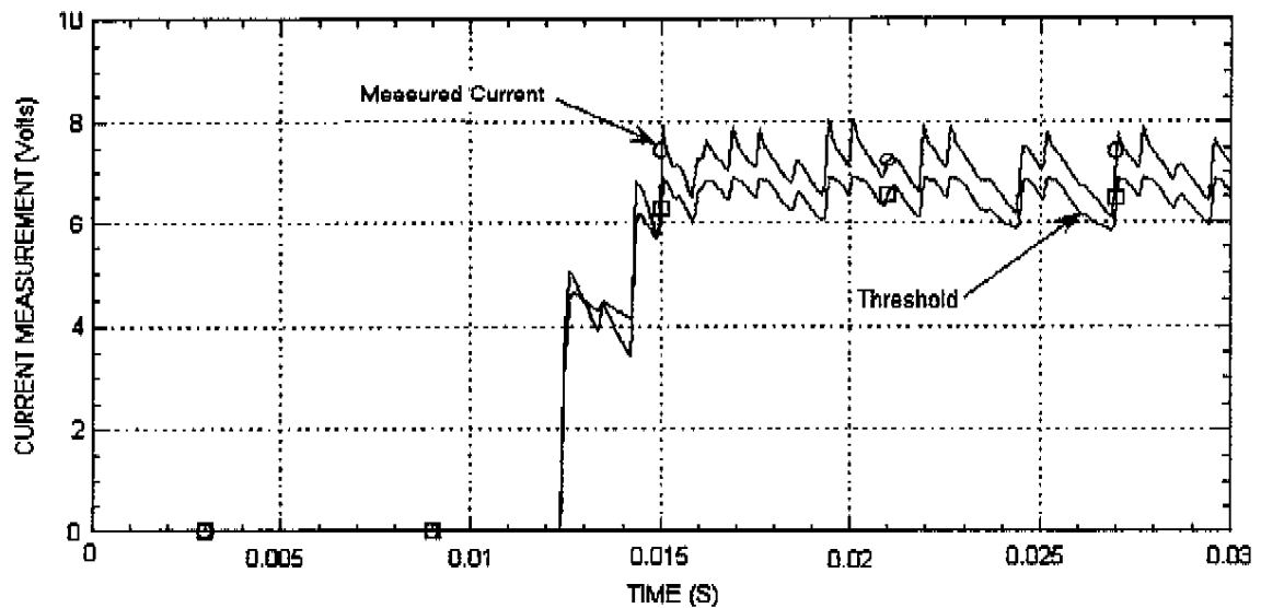
Figure 5: Measurement of Lightning Current by Relay A
