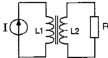
Figure 3: Interposed Current Transformer
