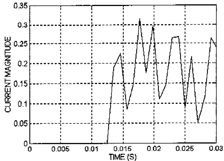
Figure 7: Digital Filter Response to Lightning
