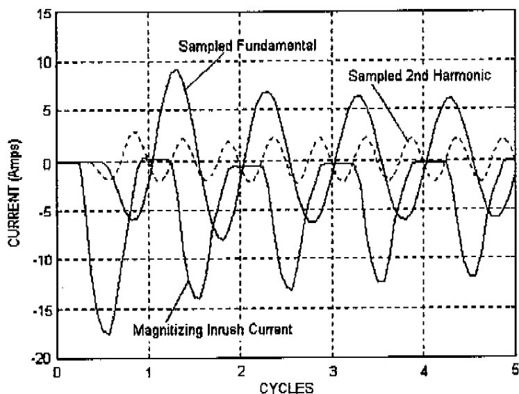
Figure 11: Transform Inrush Current
