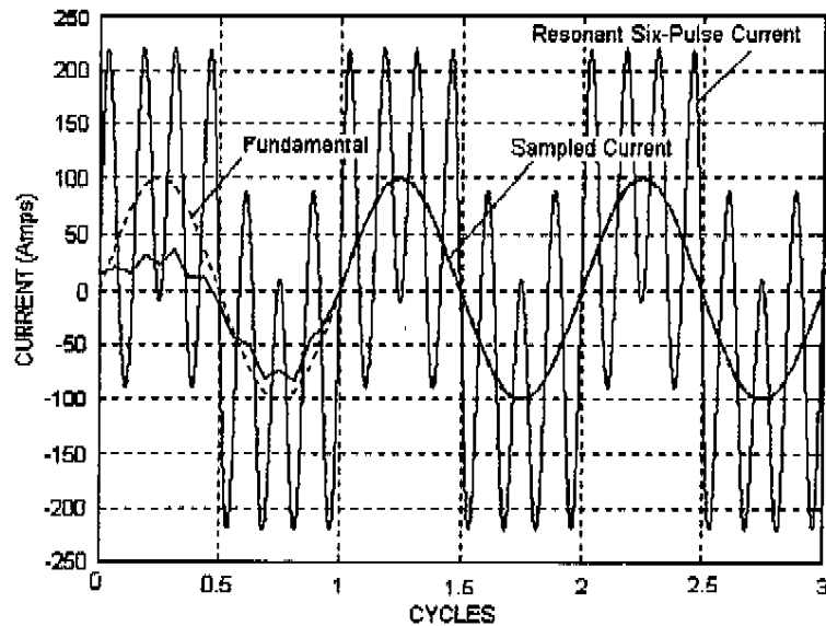
Figure 10: Digital Filtering and Fundamental of Six-Pulse Waveform With Resonance
