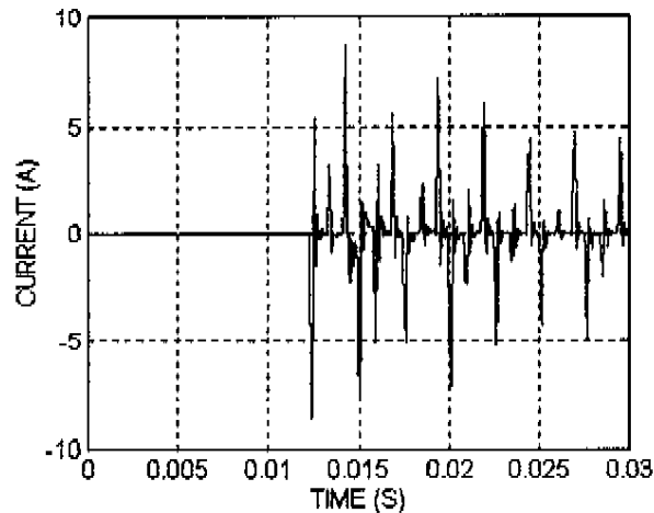
Figure 1: Current Samples Due to Lightning
