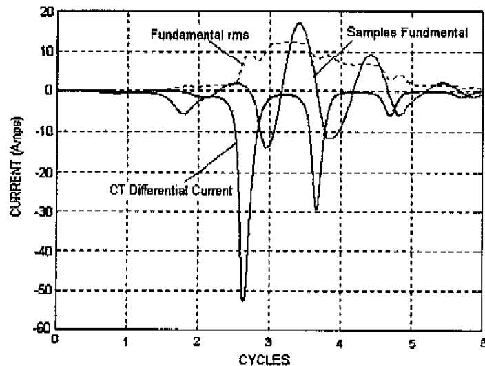
Figure 14: Differential Current and Sampled Fundamental
