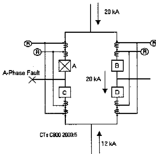
Figure 12: Ringbus Fault
