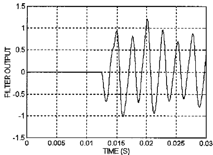
Figure 6: Response of the Anti-Aliasing Filter to Lightning
