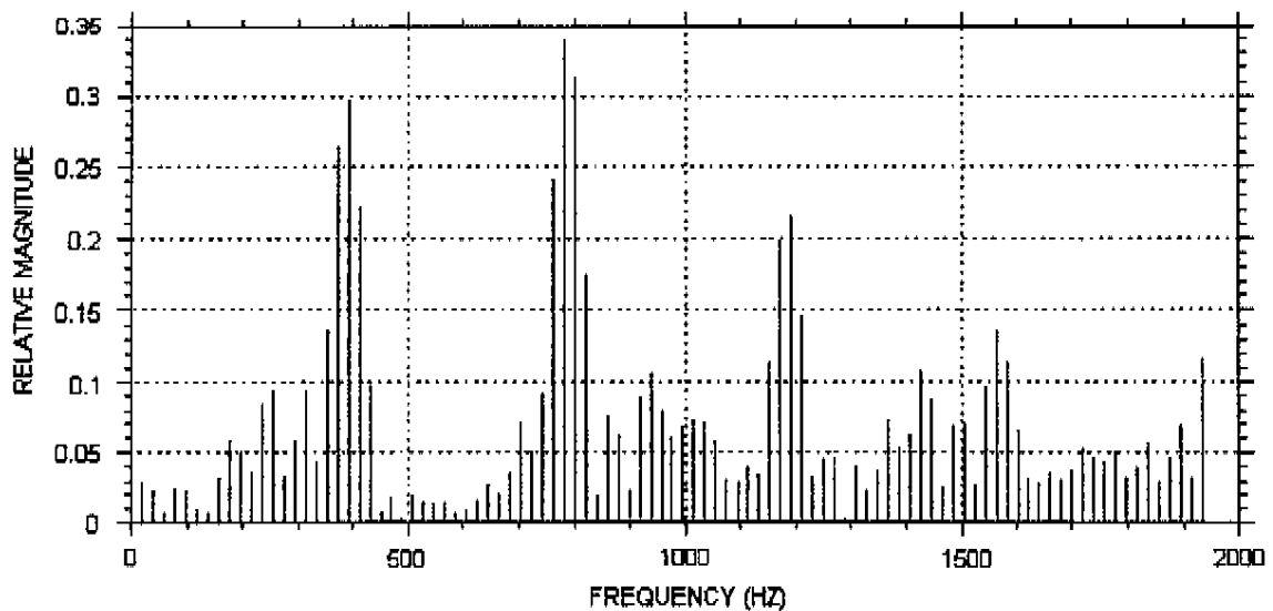
Figure 2: FFT of Current Samples
